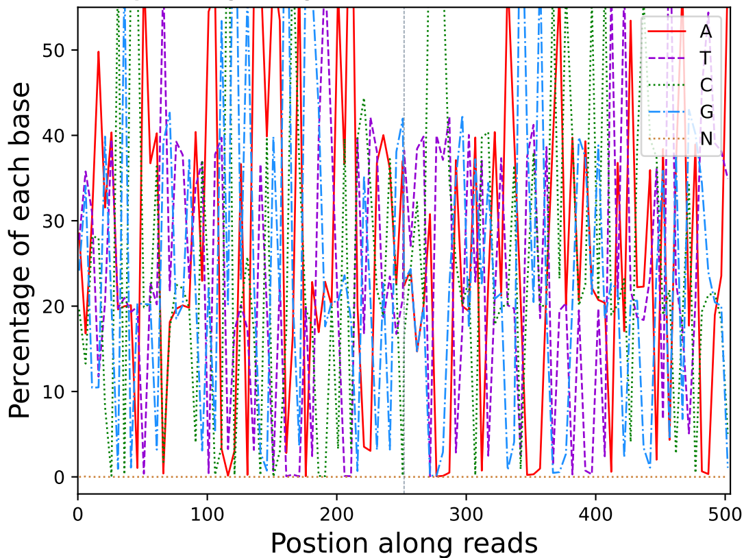
Base percentage along reads (R10901)
